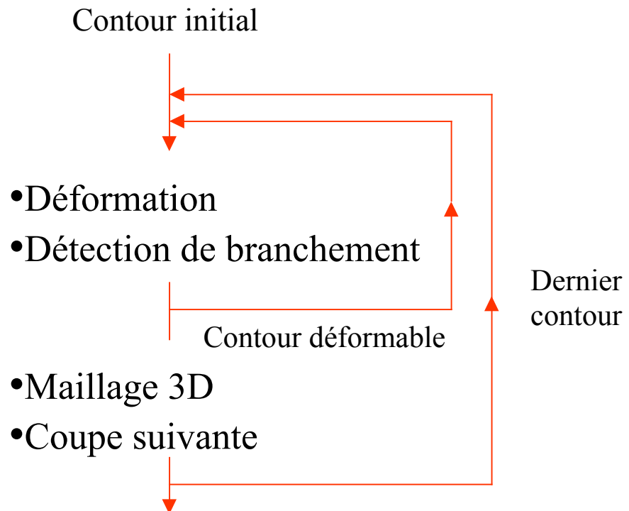
Figure 3 : Processus global de reconstruction
